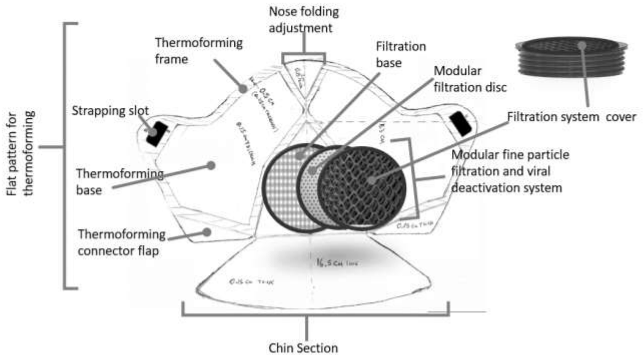
Figure 1. Flat Pattern for Thermoforming and Modular Fine Particle Filtration and viral deactivation system
