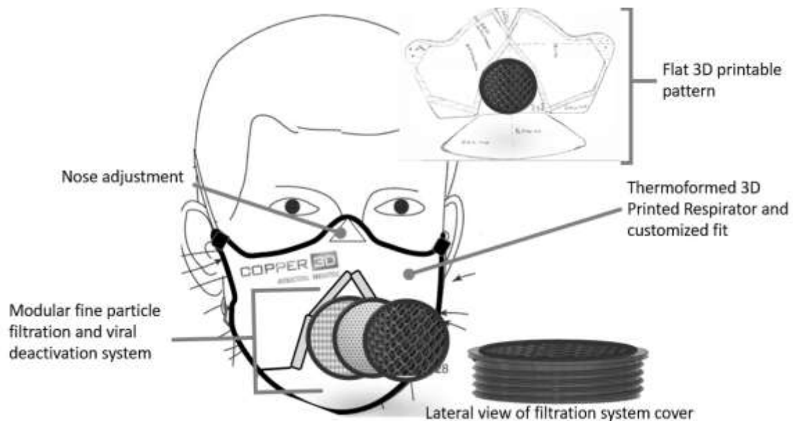
Figure 2. Thermoformed Respirator
